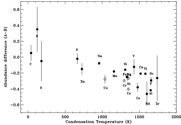
Fig. 10. Abundance difference for the components of HD 113984 as a function of the condensation temperature. From [11]
