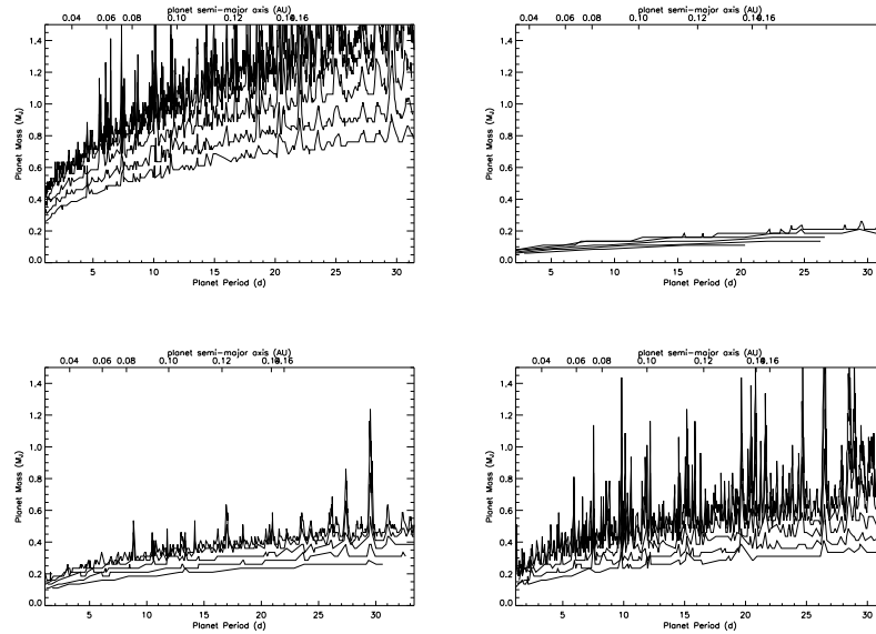
Fig. 19. Upper limits on planetary companion on short-period circular orbit for four stars representative of our sample. The different lines refer to the exclusion limits for (from top to bottom) 95%, 90%, 75%, 50%, and 25% of the planets. For the star on the upper-left corner planet detectability is strongly limited by stellar activity. The star in the upper-right corner is the one with the best limits, thanks to the low dispersion of RVs and the large number of measurements. The behaviour of the other two stars is more typical for our survey. The 'noisy' run of exclusion limits with period for the star in the lower-right corner is due to the small number of measurements.
